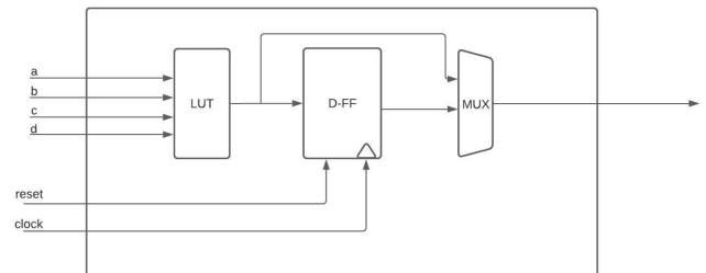
Fig. 4: CLB representation.
